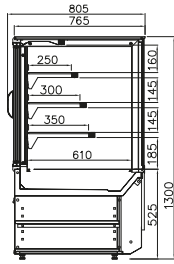
VVSTNT - VD neutra neutral neutre neutra
